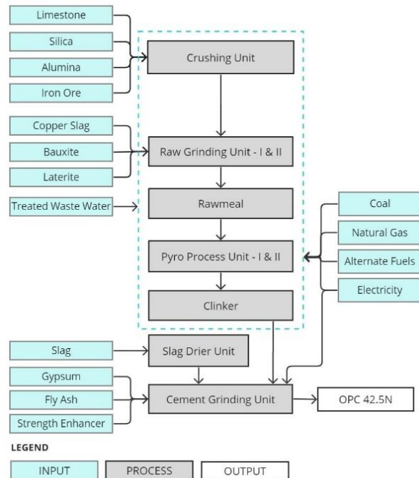
Figure 2: Unit process of OPC 42.5N
