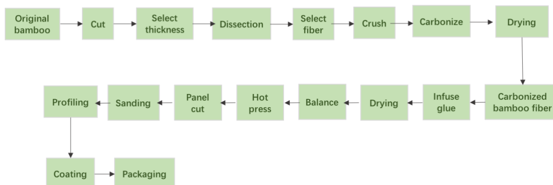
Figure 3 dasso Strand Woven Bamboo manufacturing process
