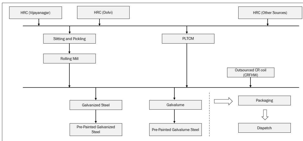
Figure 2: Manufacturing Process at Vasind
