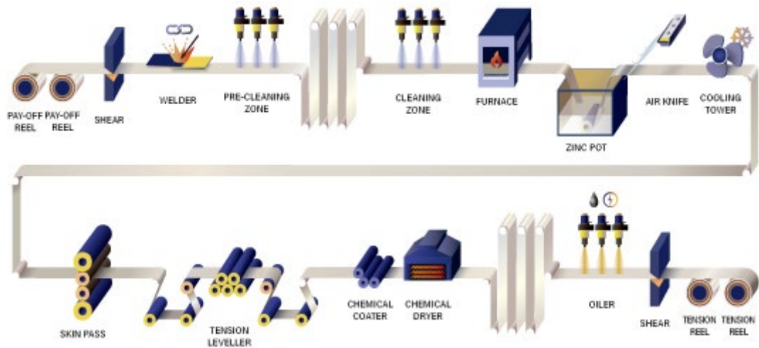
Figure 5 CGL process
