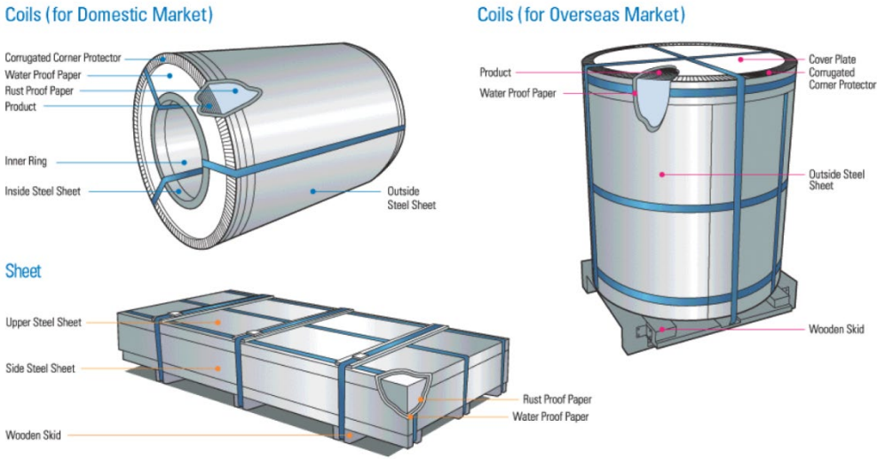
Figure 1 Product packing
