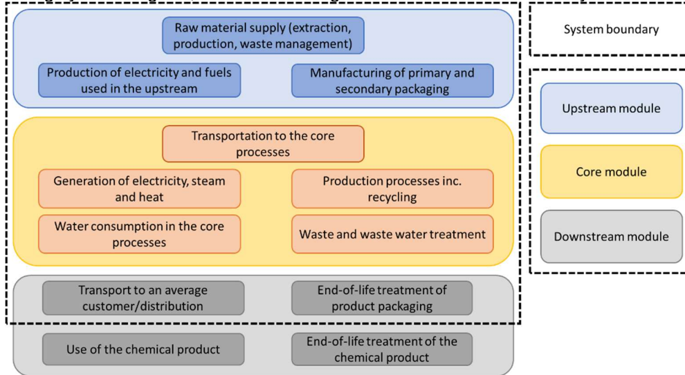
Figure 1 System boundary of the LCA study conducted on Spolsan® G produced by Spolana
