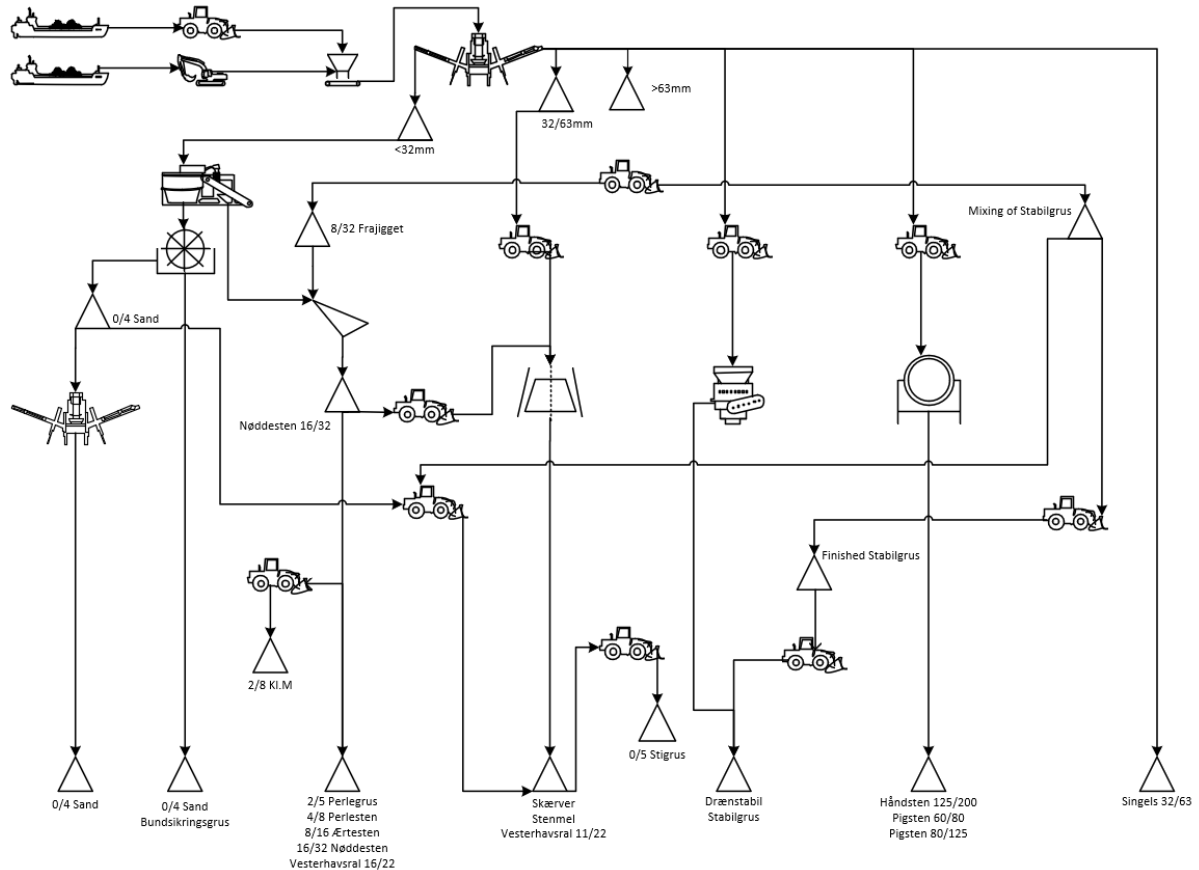
Figure 1: Process set-up for the production of aggregates at the declared site.
