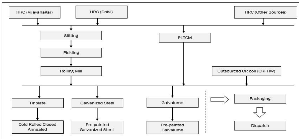
Figure 2: Manufacturing Process at Tarapur
