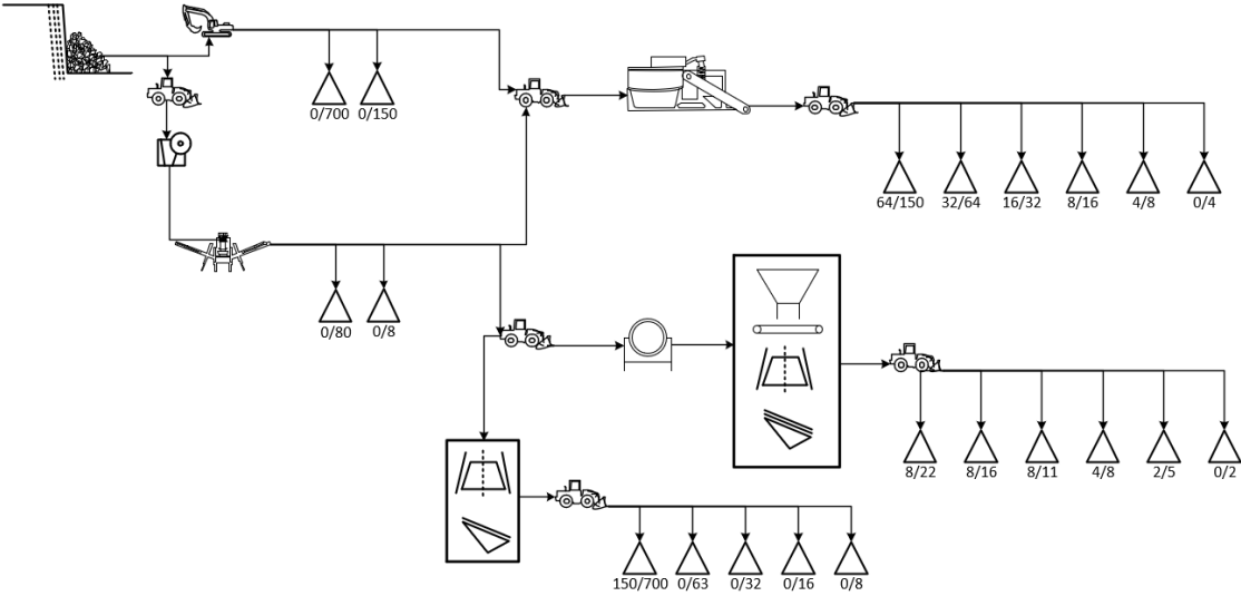
Figure 1: Process set-up for the production of aggregates at the declared site.
