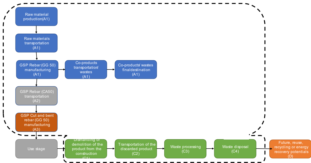
Figure 2: System boundary of the life cycle assessment for Reinforcing Steel Bar Gerdau GG 50
