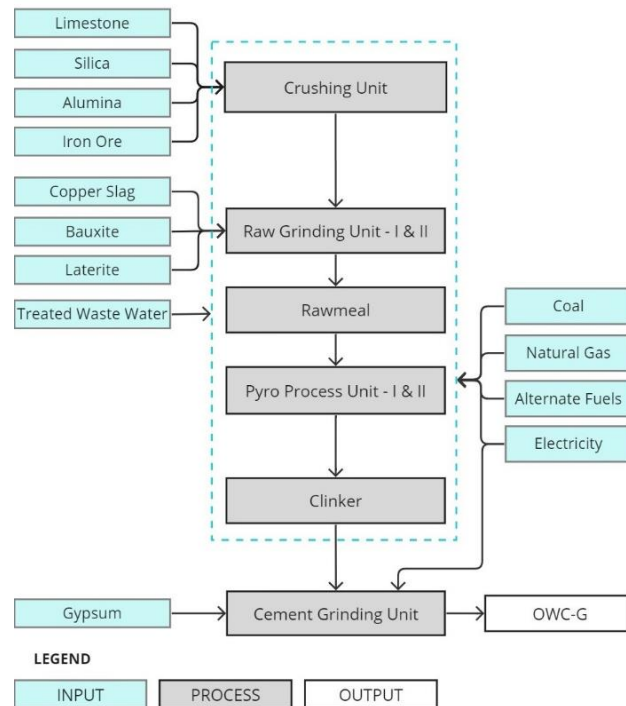
Figure 2: Unit process of OWC-G
