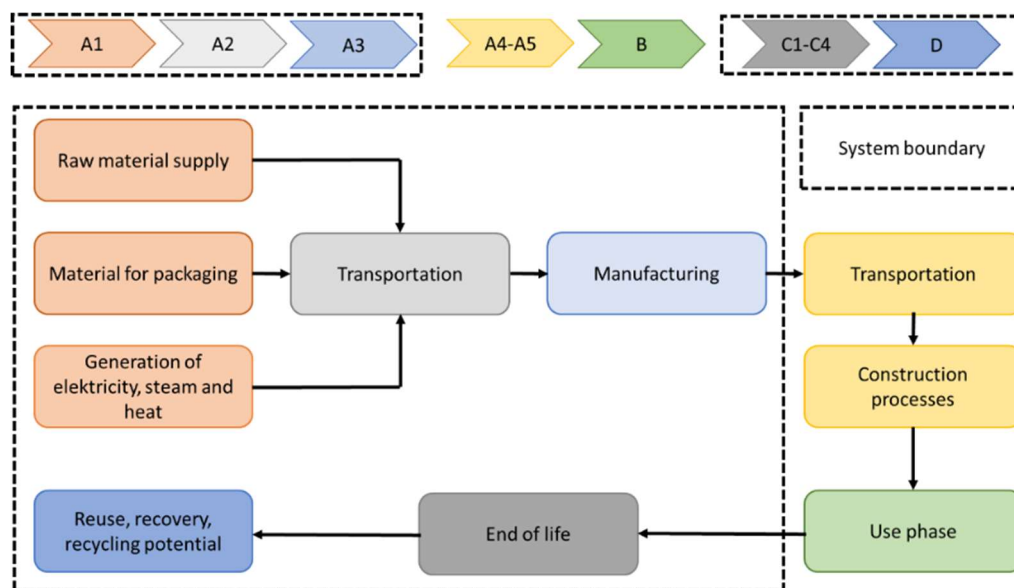
Figure 1 System Boundary of the LCA study conducted on Mini Martin luminaire produced by SIA VIZULO
