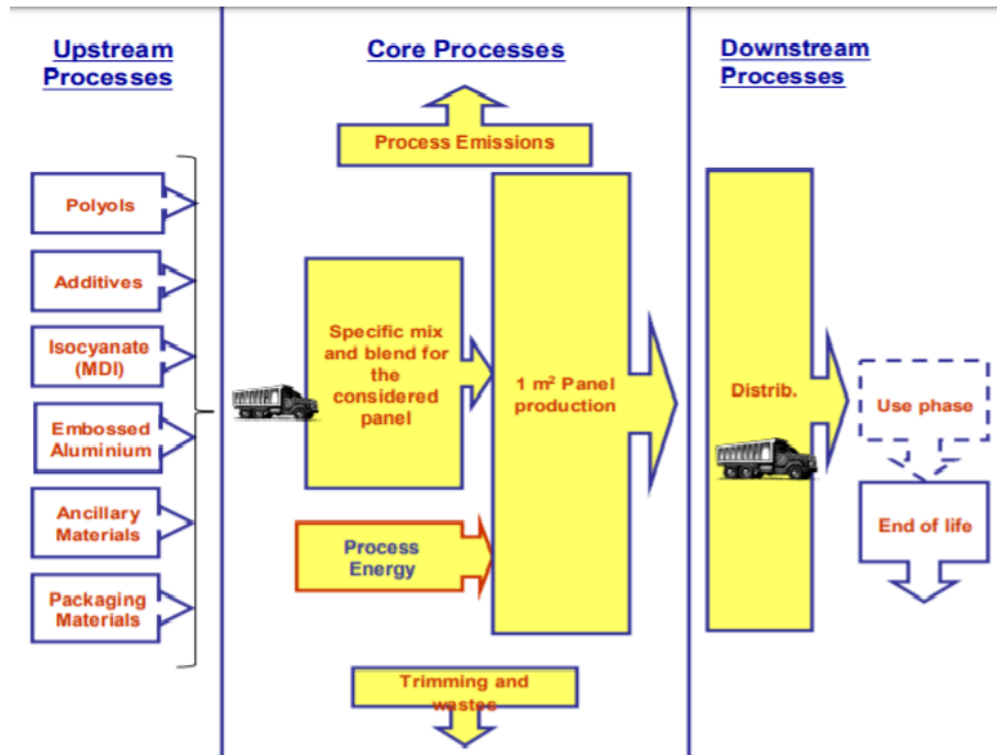
Figure 1 -- Preliminary outline of the process considered. The yellow areas show the operations carried out in P3 . The dotted lines mark phases as viewed in qualitative way.
