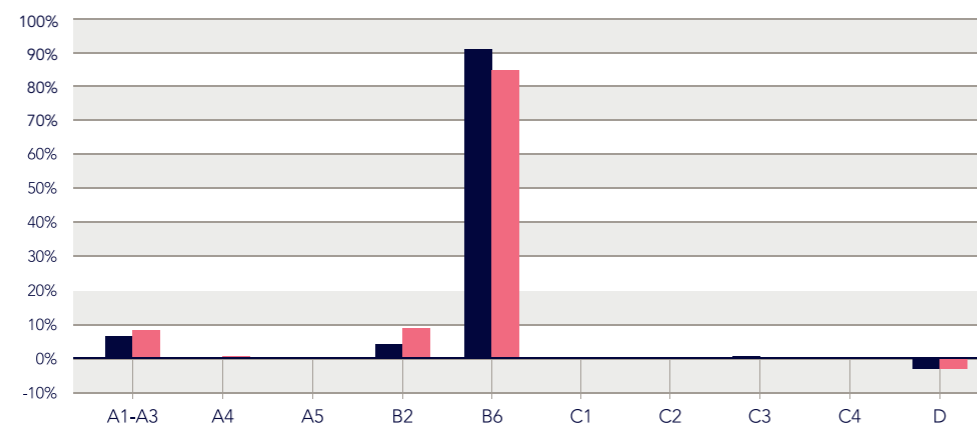
Caption: GWP - total = global warming potential; GWP - fossil = global warming potential (fossil fuel only); GWP - biogenic = global warming potential (biogenic); GWP - luluc = global warming potential (land use only); ODP = ozone depletion; AP = acidification terrestrial and freshwater; EP - freshwater = eutrophication potential (freshwater); EP - marine = eutrophication potential (marine); EP - terrestrial = eutrophication potential (terrestrial); POCP = photochemical ozone formation; ADPE = abiotic depletion potential (element), ADPF = abiotic depletion potential (fossil) WDP = water scarcity.
