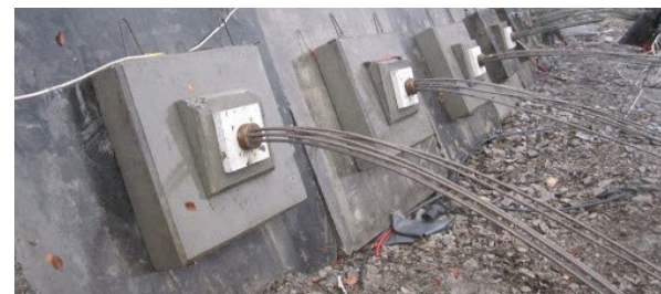
Ground and rock anchors
