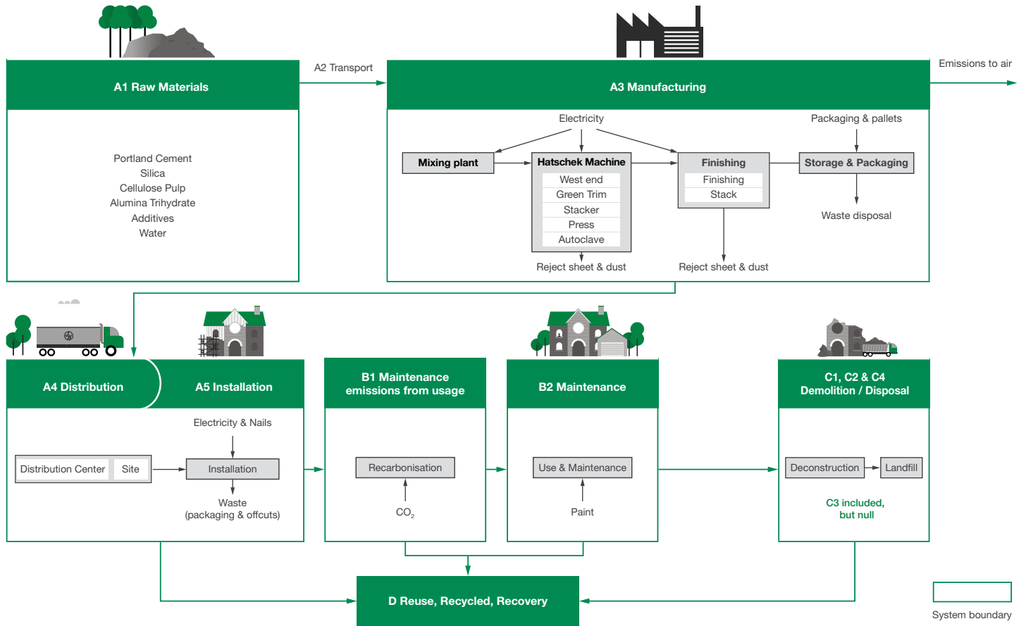
FIGURE 1. SYSTEM BOUNDARY
