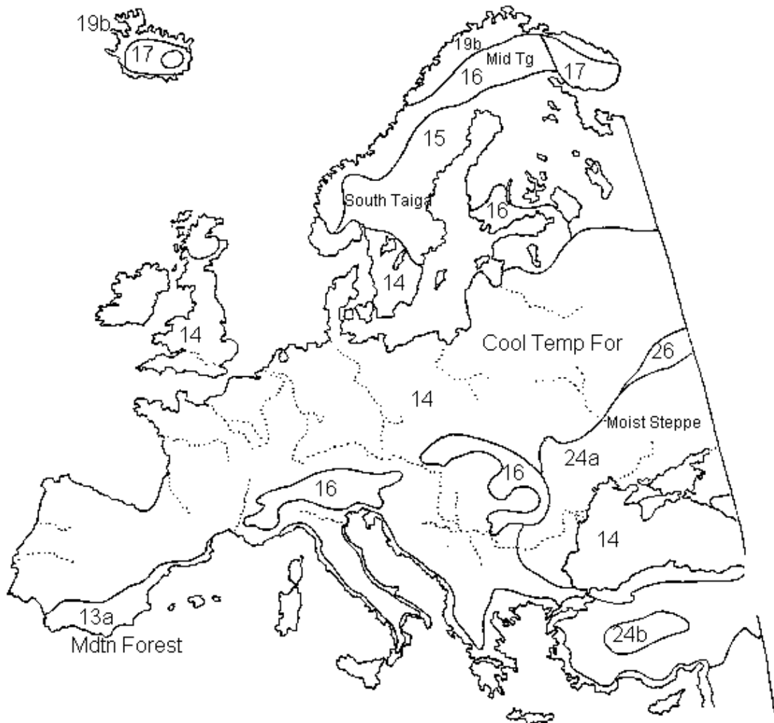
Reconstructed vegetation cover for both 5000 C14 years ago and present potential.
