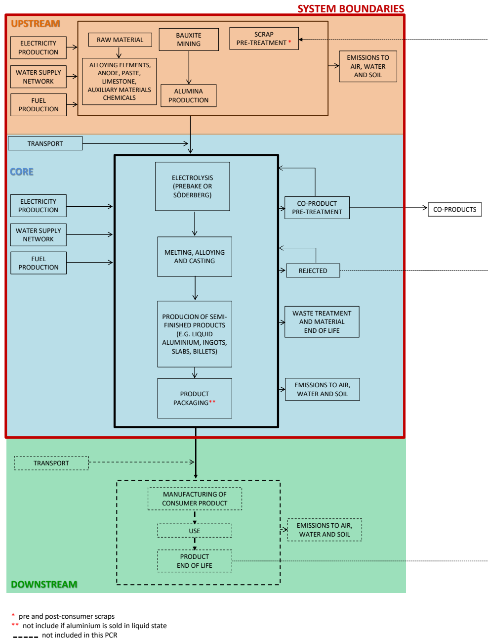
Figure 2 System diagram illustrating the processes for primary aluminium, that shall be included in the product system, divided into upstream, core and downstream processes. The illustration of processes to include may not be exhaustive. If any omission of life-cycle stages and processes are made, the system diagram should indicate it.
