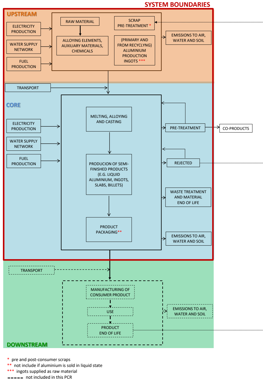
Figure 3 System diagram illustrating the processes for aluminium from recycling, that shall be included in the product system, divided into upstream, core and downstream processes. *** in some cases, aluminium (e.g. ingots from recycling and/or primary) is supplied and melted in core with other elements to obtain the final product. The illustration of processes to include may not be exhaustive. If any omission of life-cycle stages and processes are made, the system diagram should indicate it.
